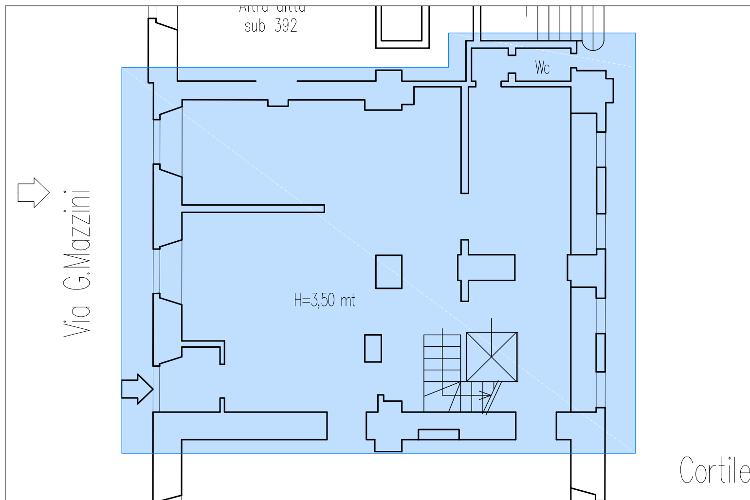
PIANO TERRENO
